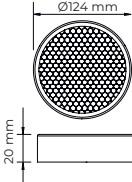
L016 Louver honeycomb PAR38
