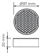
L015 Louver honeycomb PAR30
